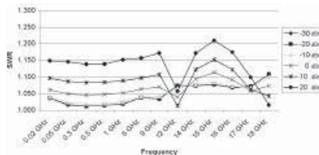
Figure 2. Typical SWR for the E9322A and E9326A sensors at various power levels
