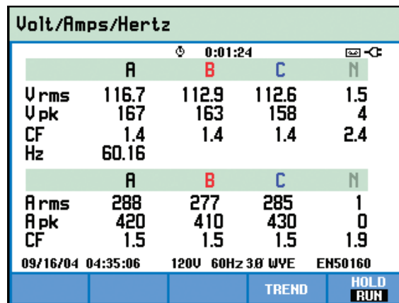
Figure 2. Recording all phase voltages and neutral to ground voltage is a good start for a PQ analysis of critical equipment and overall distribution system health.
