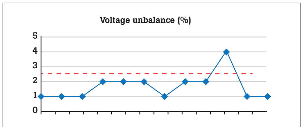
Figure 1. This maintenance control chart tracking voltage unbalance shows a Nov-03 reading above the 2.5 % limit and then the effect of the corrective action.
