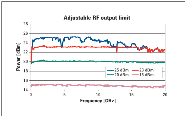
RF output limit (measured)
