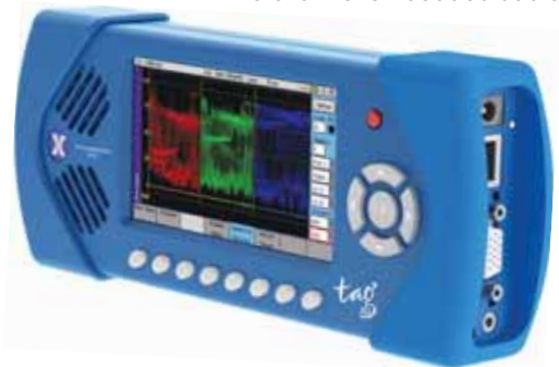
Sx TAG Combined analyser-monitor IP, Analogue, SDI, Optical - SFP support 16 channel embedded audio
