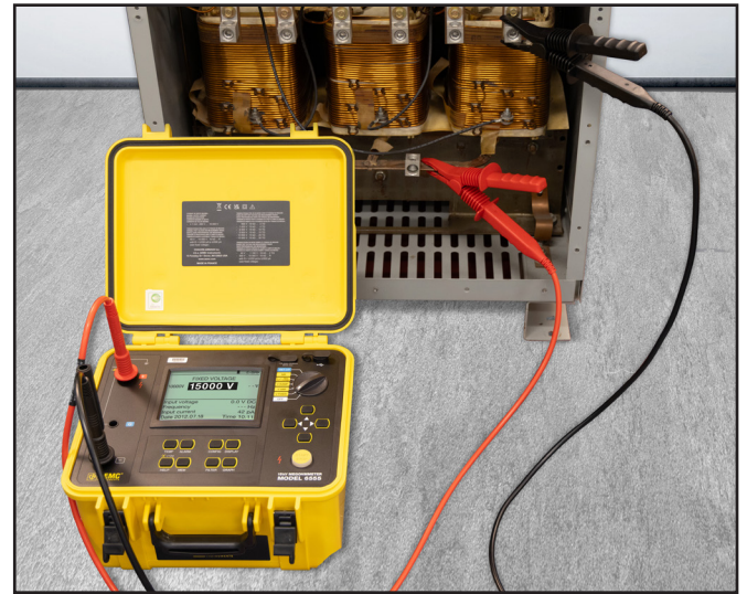
Model 6555 performing a single-phase test on a three-phase transformer.
