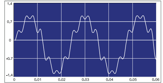
Harmonic Waveform
