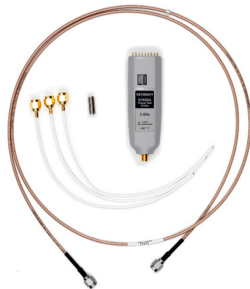
Figure 35. N7020A Power Rail Probe.
