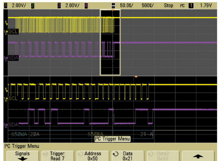
On-screen serial decode of an I 2 C packet.
