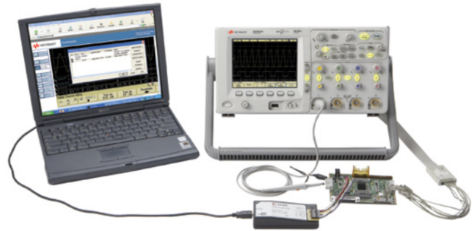
Debug and validate your FPGA designs faster and more effectively with FPGA dynamic probe and Keysight MSO.
