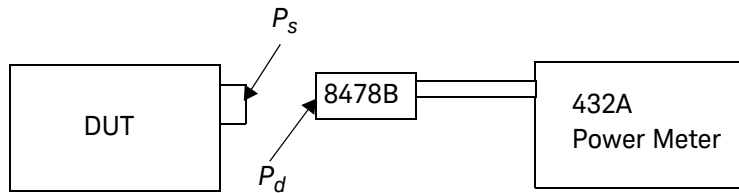
Figure C-1 Measurement Setup
