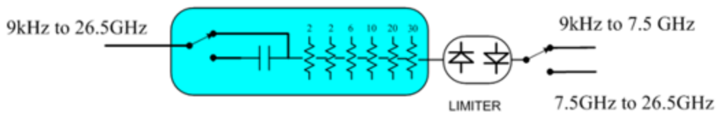
Configuration 2: Mechanical attenuator, no optional electronic attenuator
