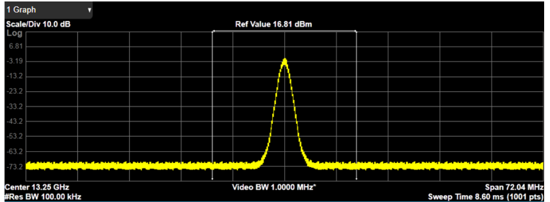
Spectrum View with Bar Graph On
