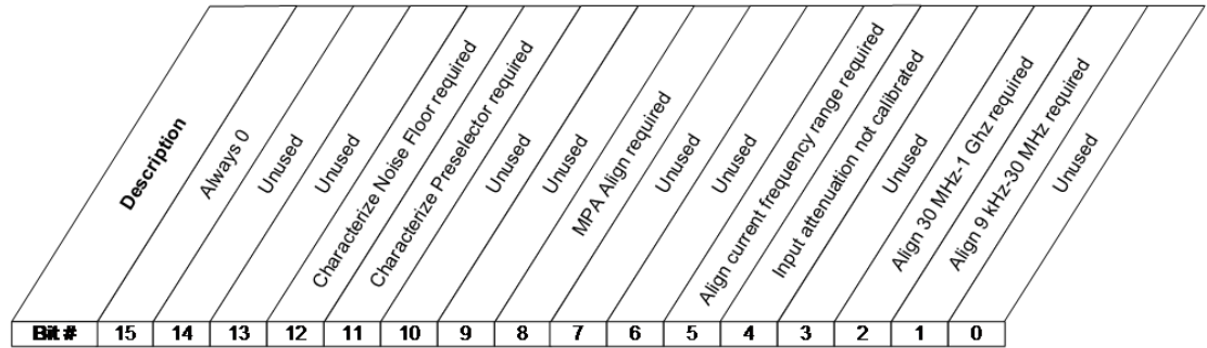
STATus:QUESTIONable:CALibration:EXTended:NEEDED Register
