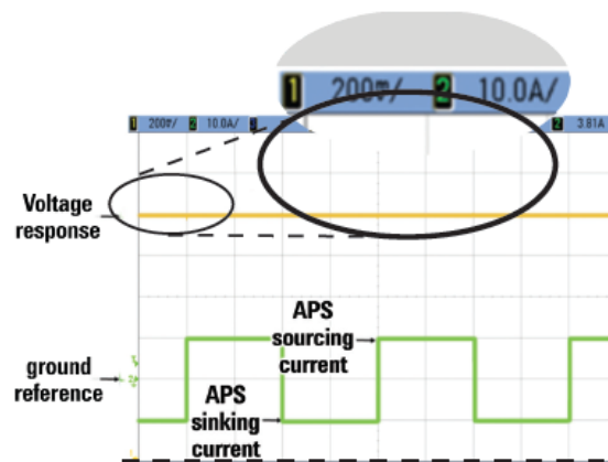
Figure 3. Shows an example of an APS power supply smoothly pulsing back and forth from sinking current at -10 A to sourcing current at 10 A. Notice that the voltage level captured at high resolution on the top trace remains constant with no glitches.
