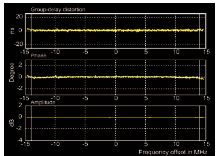
Frequency response and group-delay distortion of 50 MHz resolution filter (example).
