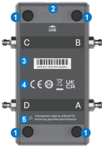
Figure 2 Rear panel
