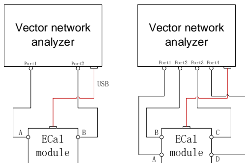
Figure 5 Connection diagram 3
